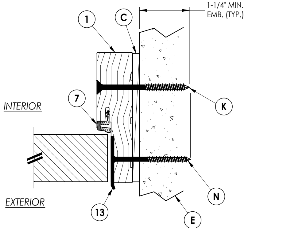
3 HORIZONTAL CROSS SECTION 3 Shown Direct to masonry Outswing Shown (Inswing Similar)
