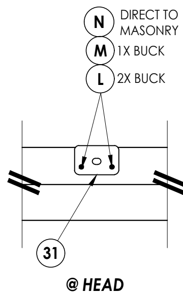
ASTRAGAL BOLT STRIKE DETAIL
